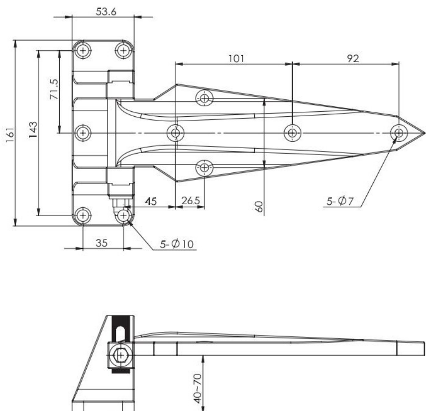
鋅合金，鍍鉻 Zinc die, Bright chrome plated
