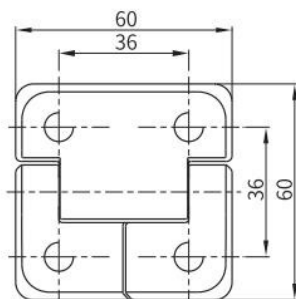
M8鑲嵌螺柱 With Threaded Studs M8
