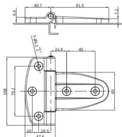
黑色PA+GF鉸鏈, 不銹鋼銷軸 Hinge Polyamide GF 30% black, M.S. zinc plated pin
