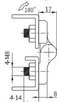
M8鑲嵌螺柱 With Threaded Studs M8
