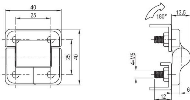
M5 鑲嵌螺柱 With Threaded studs M5
