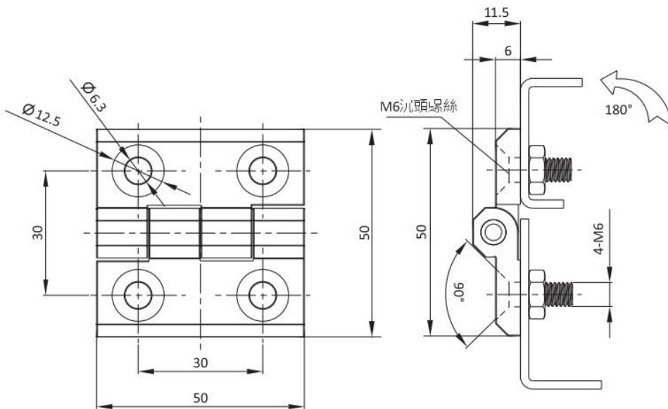
M6 沉頭螺絲固定 Countersunk Screw M6
