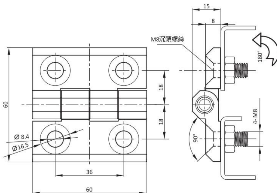
M8 沉頭螺絲固定 Countersunk Screw M8
