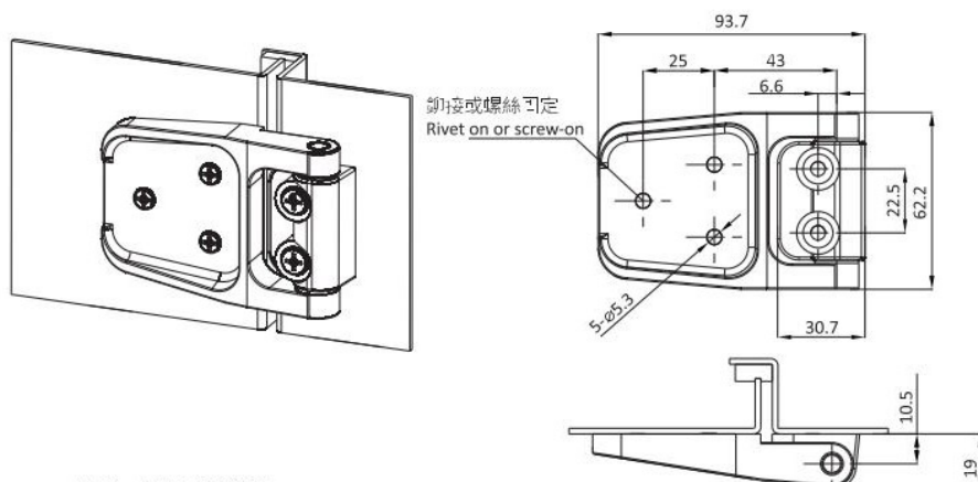
黑色PA+GF鉸鏈, 鍍鋅鋼銷軸 Hinge Polyamide GF 30% black, M.S. zinc plated pin
