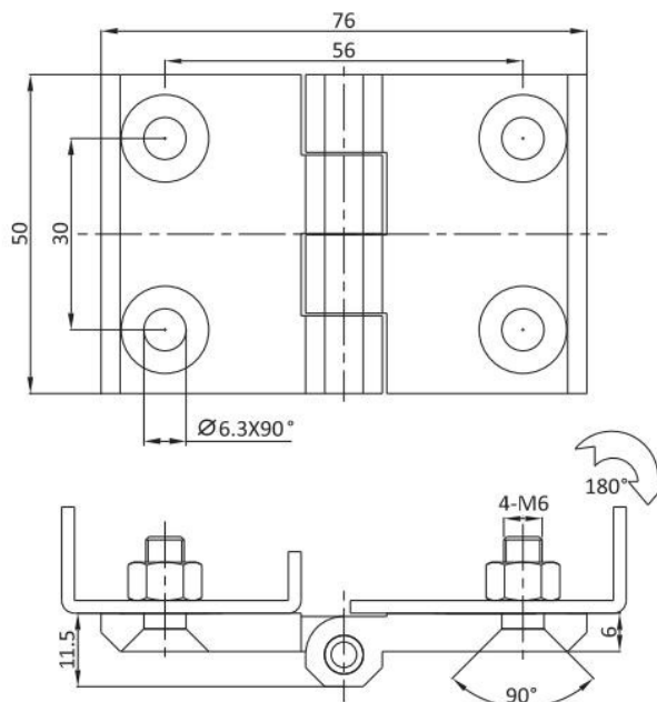
M6 沉頭螺絲固定 Countersunk Screw M6
