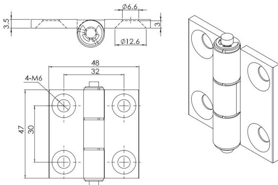
螺絲固定鉸鏈 Screw-on Hinge
