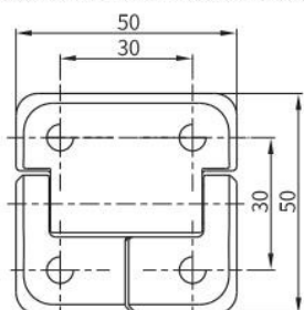
M6鑲嵌螺柱 With Threaded Studs M6
