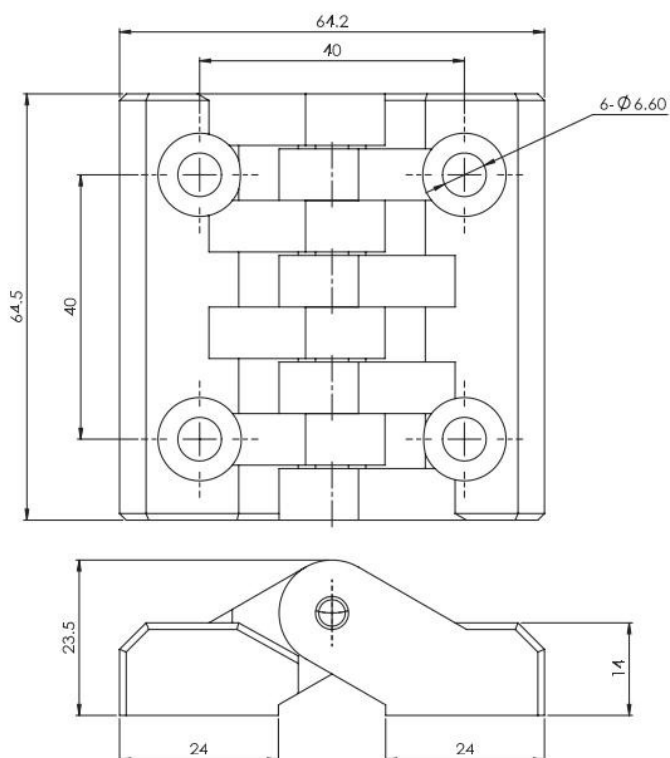
黑色PA螺絲固定鉸鏈,鍍鋅鋼銷軸 Screw-on hinge polyamide GF black, pin M.S. zinc plated
