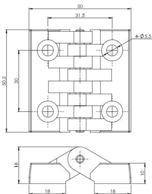
黑色PA螺絲固定鉸鏈,鍍鋅鋼銷軸 Screw-on hinge polyamide GF black, pin M.S. zinc plated
