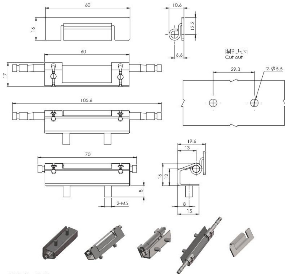
鋼鐵或不銹鋼304 Steel or stainless steel 304
