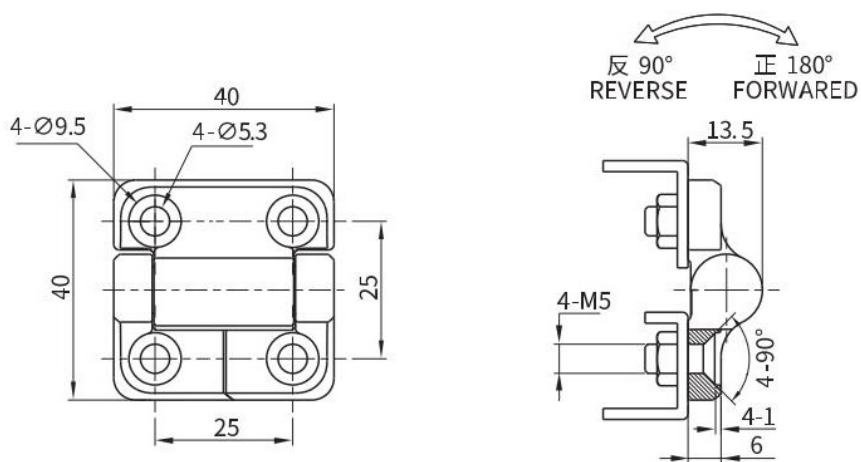
M5沉頭螺絲固定 Countersunk Screw M5
