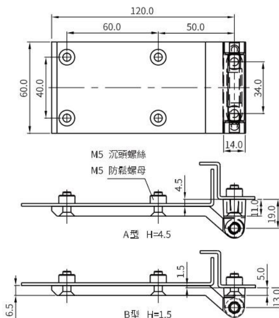
鋅合金螺絲固定鉸鏈,不鏽鋼銷釘,PA襯套 Screw-on hinge zinc die, pin stainless steel and bushes polyamide
