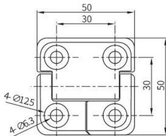
M6鑲嵌螺柱 With Threaded Studs M6
