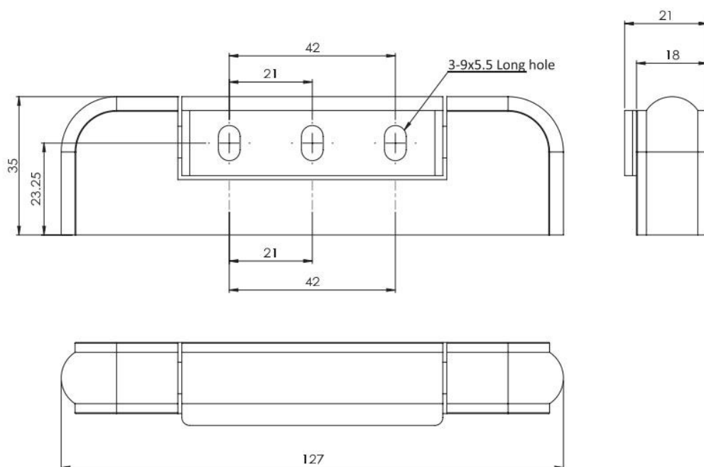
鋅合金, 鍍鉻 Zinc die, Bright chrome plated
