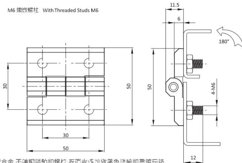
螺絲固定鉸鏈 Screw-on Hinge 50x50
